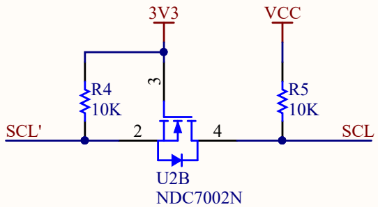
LEVEL SWITCH
