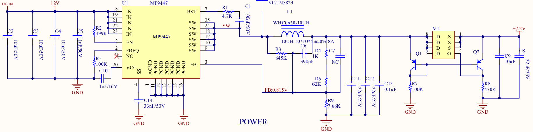
DC BUCK Adapter (7.2V)
