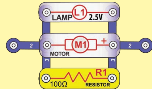
Parallel Circuit
